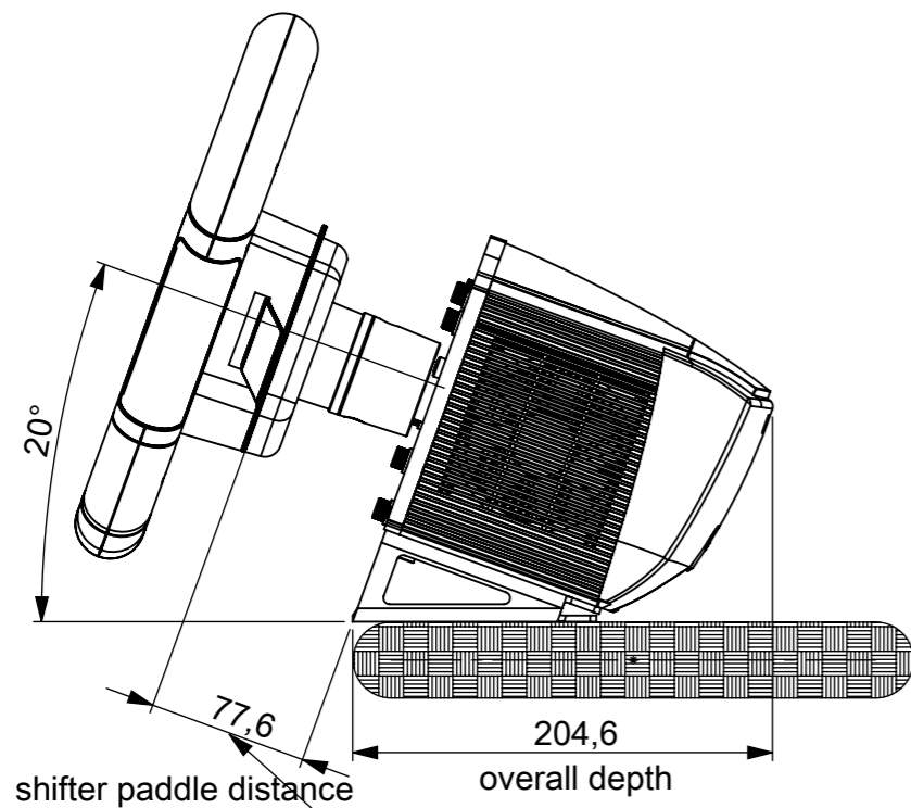
CSR Elite right side view
