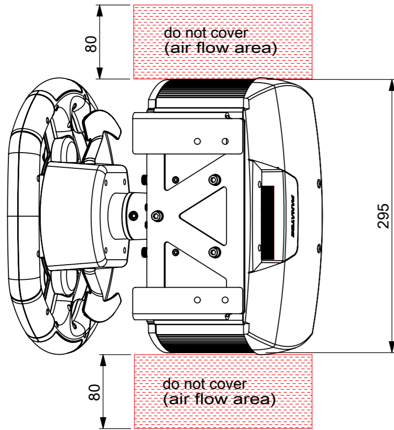
CSR Elite bottom view
